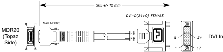
A31-00735-5012 (VLG-1/1) cable assembly
