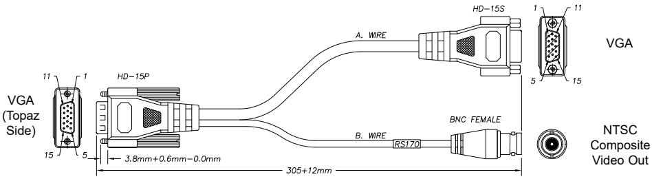
A31-00735-3012 (VLG-2/1) cable assembly
