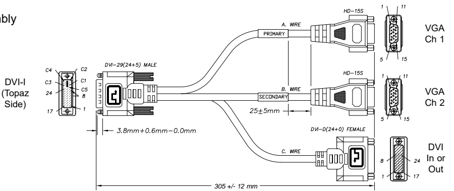
A31-00735-1012 (VLG-3/1) cable assembly
