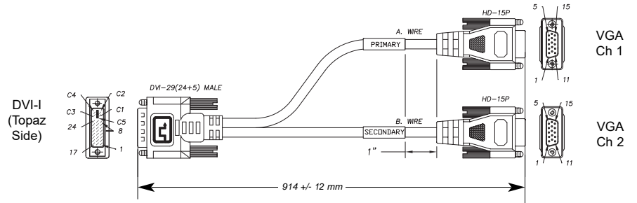
A31-00735-1011 (VLG-2/3) cable assembly
